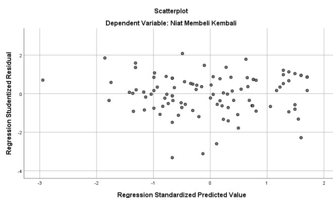
Gambar 1. Scatterplot
