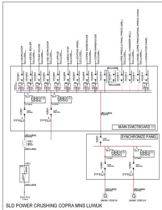
Gambar 1. Single Line Diagram Power Crushing Copra MNS Luwuk
